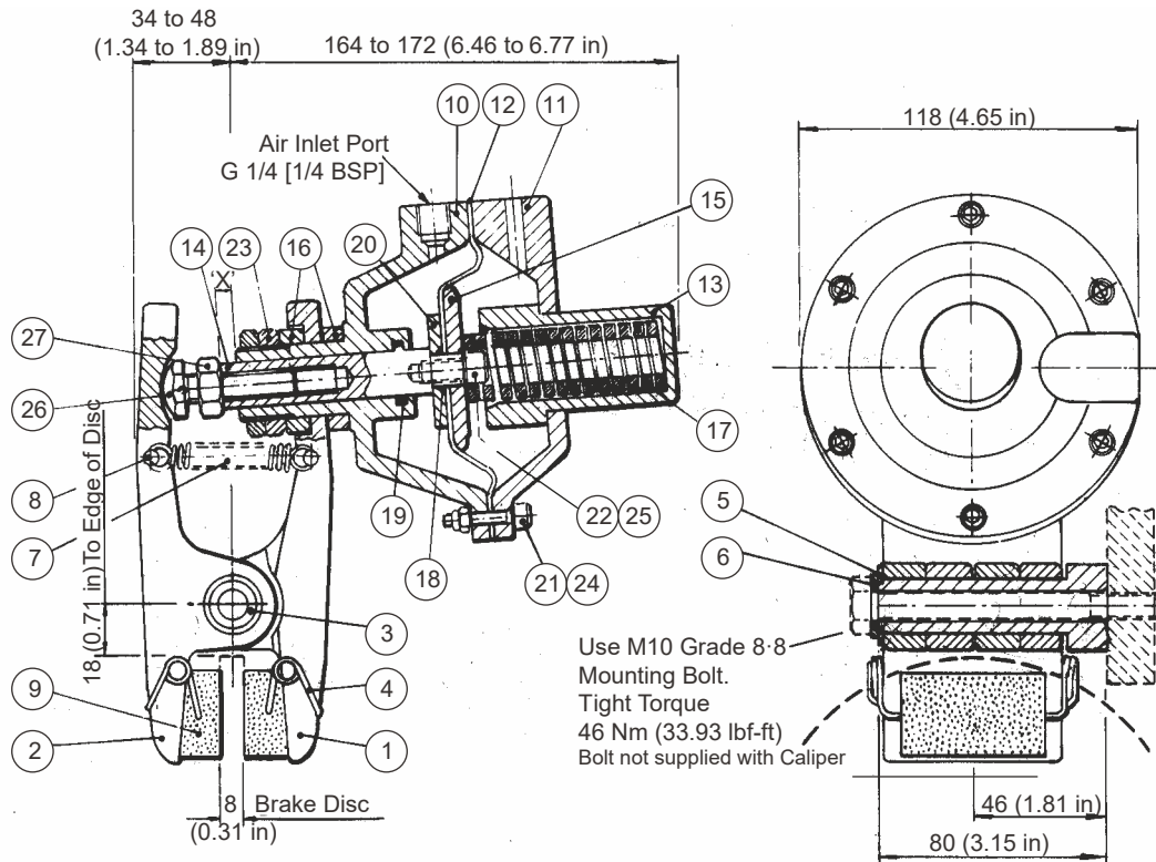
Disc Brake Caliper Assembly Type MUS4
